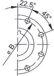
8-hole flange
