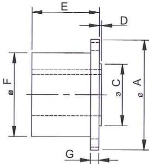
"SF" STYLE Standard flange
