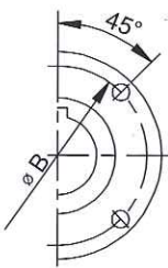
4-hole flange
