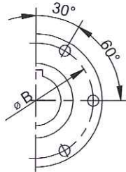
6-hole flange
